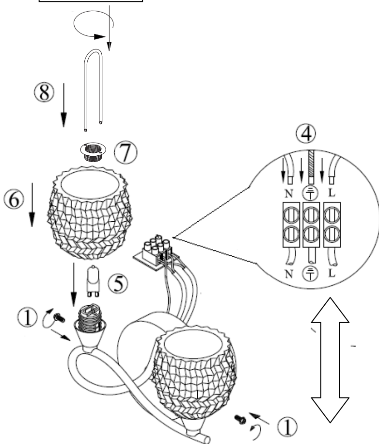
Wiring Details
