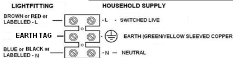
Wiring Details
